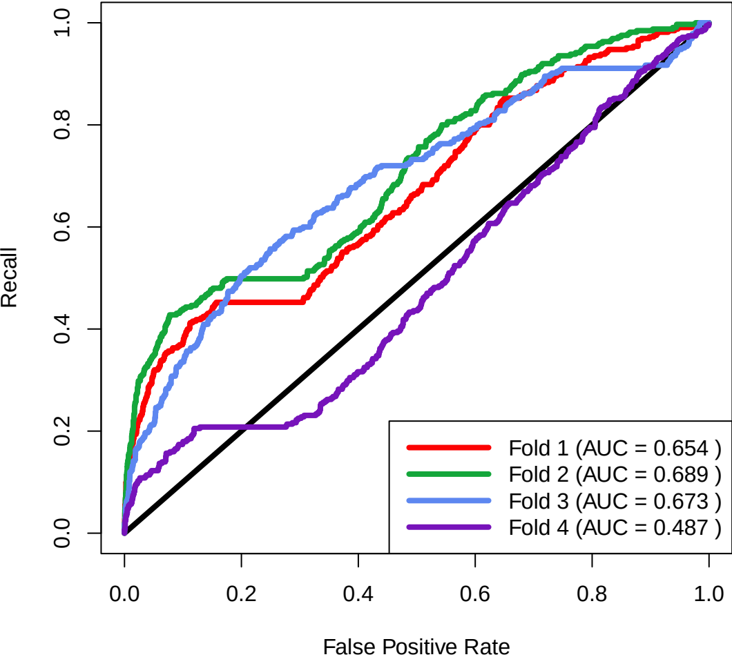
SPELL Network 430 Dataset: 430x20x10x1 Batch 50 lr 0.1 Validation
